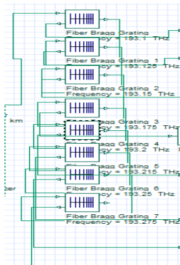
Fig. 3. Internal structure of Demux subsystem
