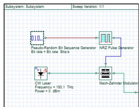
Fig. 2. Internal structure of transmitter subsystem
