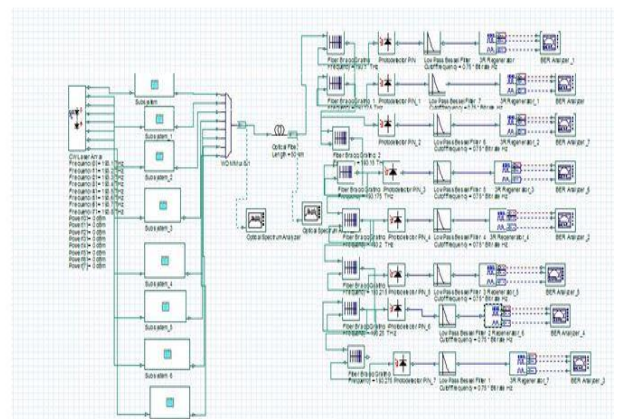
Fig. 1. Circuit diagram of FBG based demux of Bessel filter
