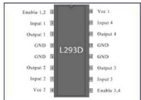
Fig.5: Motor Driver L293D
