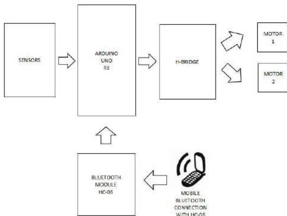
Fig.1: Block Diagram of Line following and obstacle
