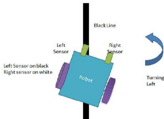
Fig.9: If left sensor comes on black line then robot turn left side.
