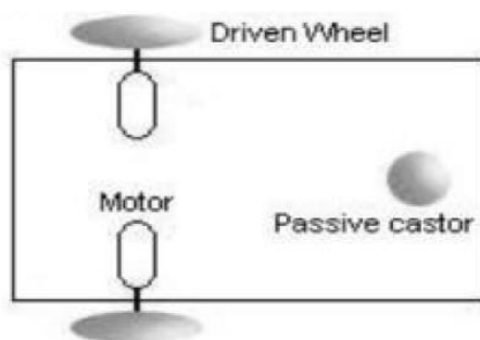
Fig.2: The Chassis
