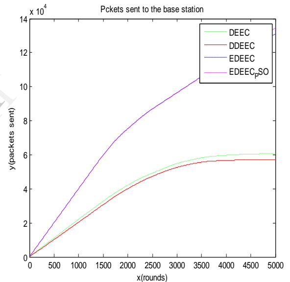
Fig. 1.5 Data reach to the Base Station Comparison
