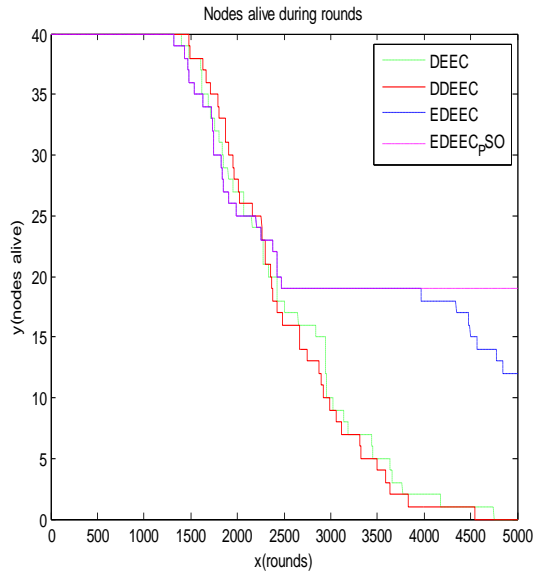
Fig. 1.2 Alive Nodes Comparison
