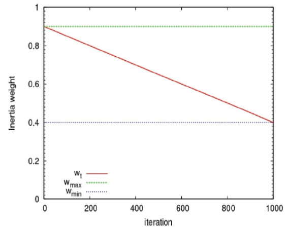
Fig.1.1 The value of the inertia weight is decreased during a run.
