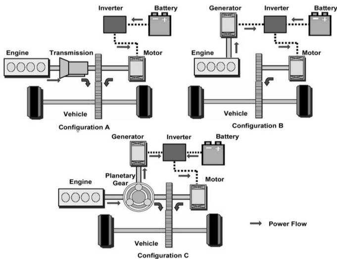
Fig. 2. Hybrid vehicle configurations
