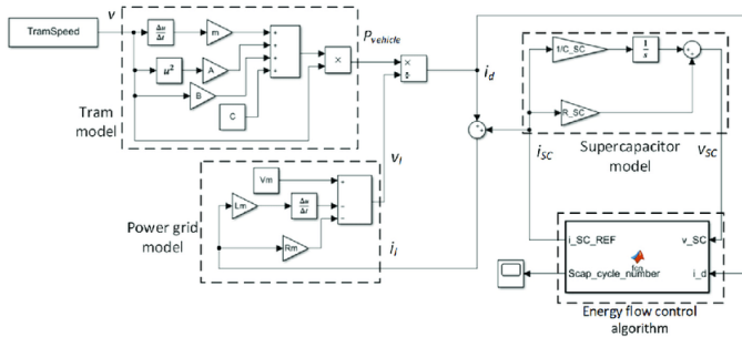
Fig. 11. Simulation Model of the Regenerative Braking System
