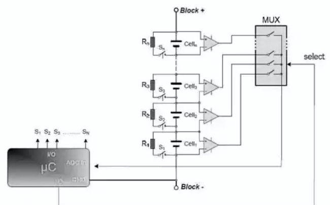
Fig. 9. Cell Balancing
