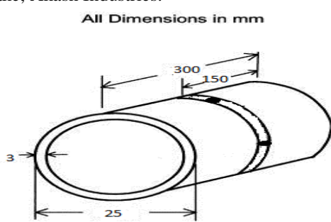
Fig. 2. Sample specimen with dimension
