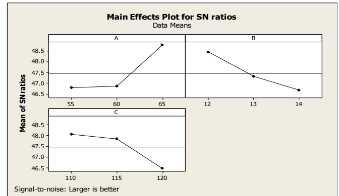
Fig. 4. Main Effects Plot for UTS
