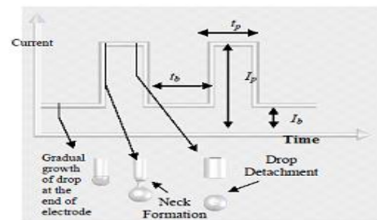
Fig. 1. Metal transfer phenomenon
