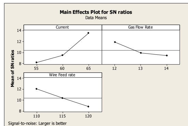
Fig. 5. Main Effects plots for Percentage of Elongation
