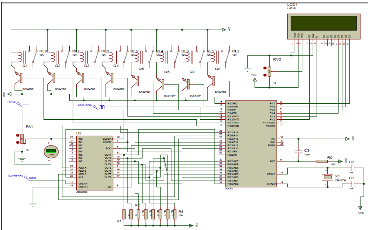
Fig 5 Simulation circuit of microcontroller-based relay operated capacitor switching
