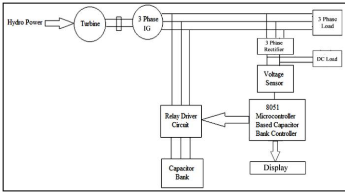
Fig. 4. Block diagram of microcontroller-based relay operated capacitor switching
