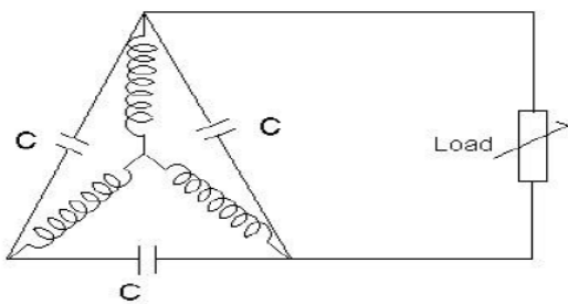
Fig. 2. Delta-connected capacitor configuration
