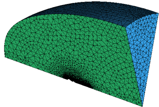
Fig.5 Mesh 30° sector
