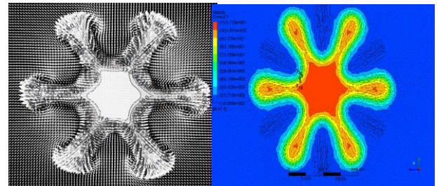
Fig.6 Velocity field at 20mm of DP-SPIV and numerical model respectively
