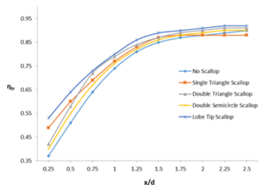
Fig.14 Mixing effectiveness of lobed nozzles along x-direction
