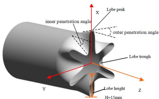
Fig.2 Six lobed nozzle used in DP-SPIV experiment
