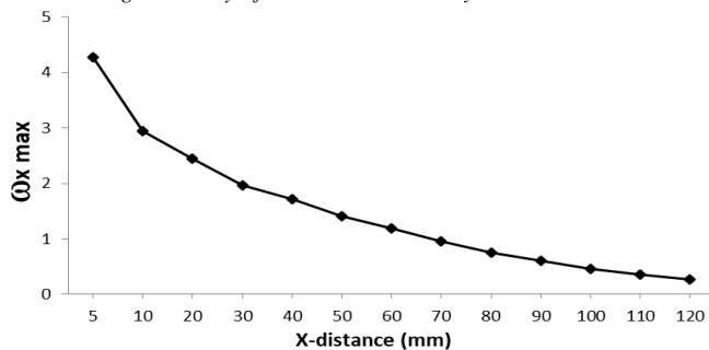
Fig.11 Decay of normal vorticity in numerical model
