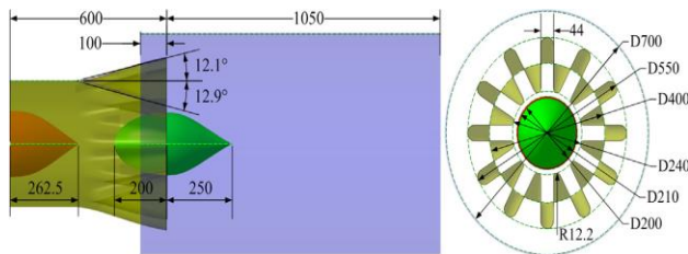
Fig.3 Lobed Nozzle with dimensions
