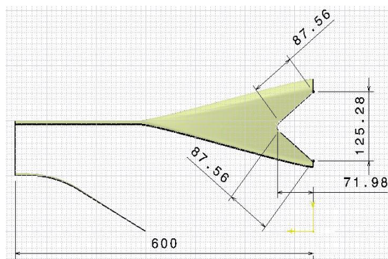
Fig.3 Lobed Nozzle with dimensions
