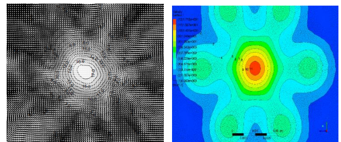
Fig.8 Velocity field at 120mm of DP-SPIV and numerical model respectively
