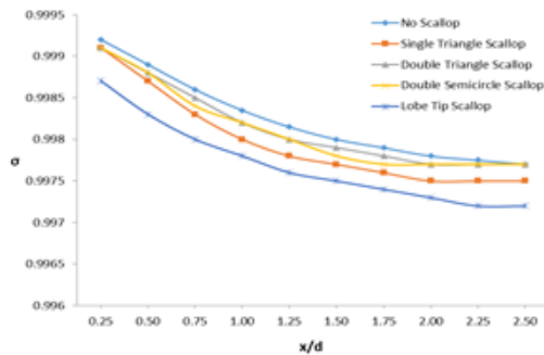
Fig.15 Total pressure recovery coefficient of nozzles along x-direction
