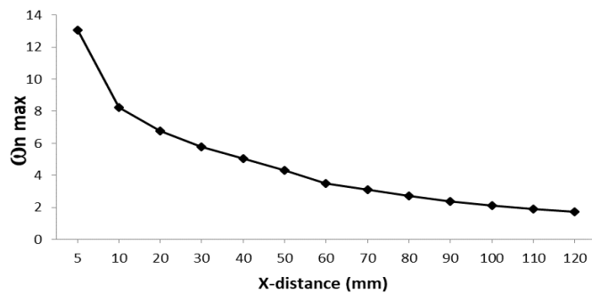
Fig.10 Decay of streamwise vorticity in numerical model
