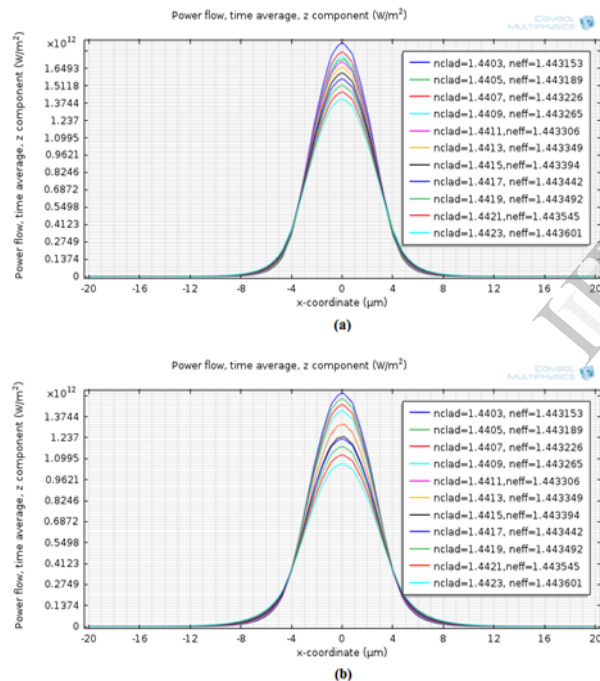
Figure 8. Variation of power flow with radial distance from fibre core centre for (a) \lambda=1310 nm and (b) \lambda=1550 nm [note: figure in colour].
