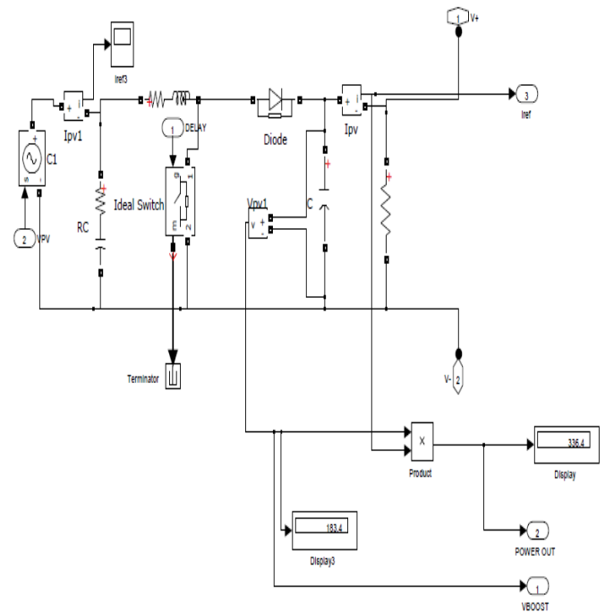
Fig 11: Boost Converter
