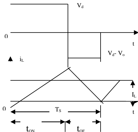
Fig 6: Wave Forms
