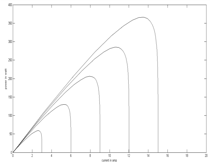
Fig 3: PV Characteristics
