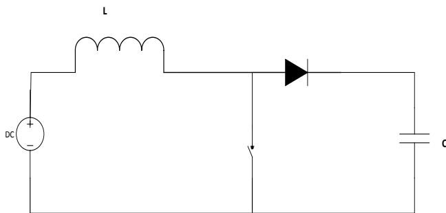
Fig 5: Boost Converter
