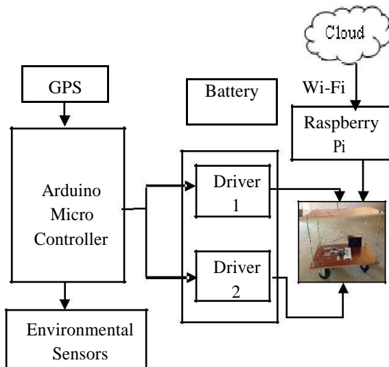
Fig.2. Mobile Robot Control Architecture
