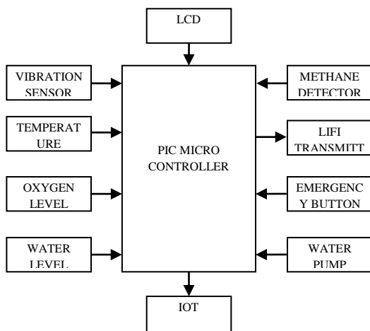
Fig 3: Transmitting Section
