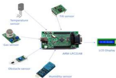
Fig 12: System Architecture
