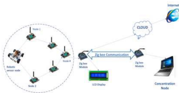
Fig 13: Concentration Node
