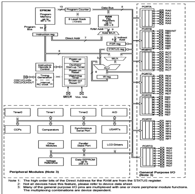
Fig 4: Basic Block Diagram Of PIC Microcontroller
