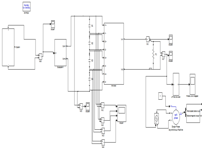
Fig 2 Simulation circuit for 9-level Cascaded Inverter
