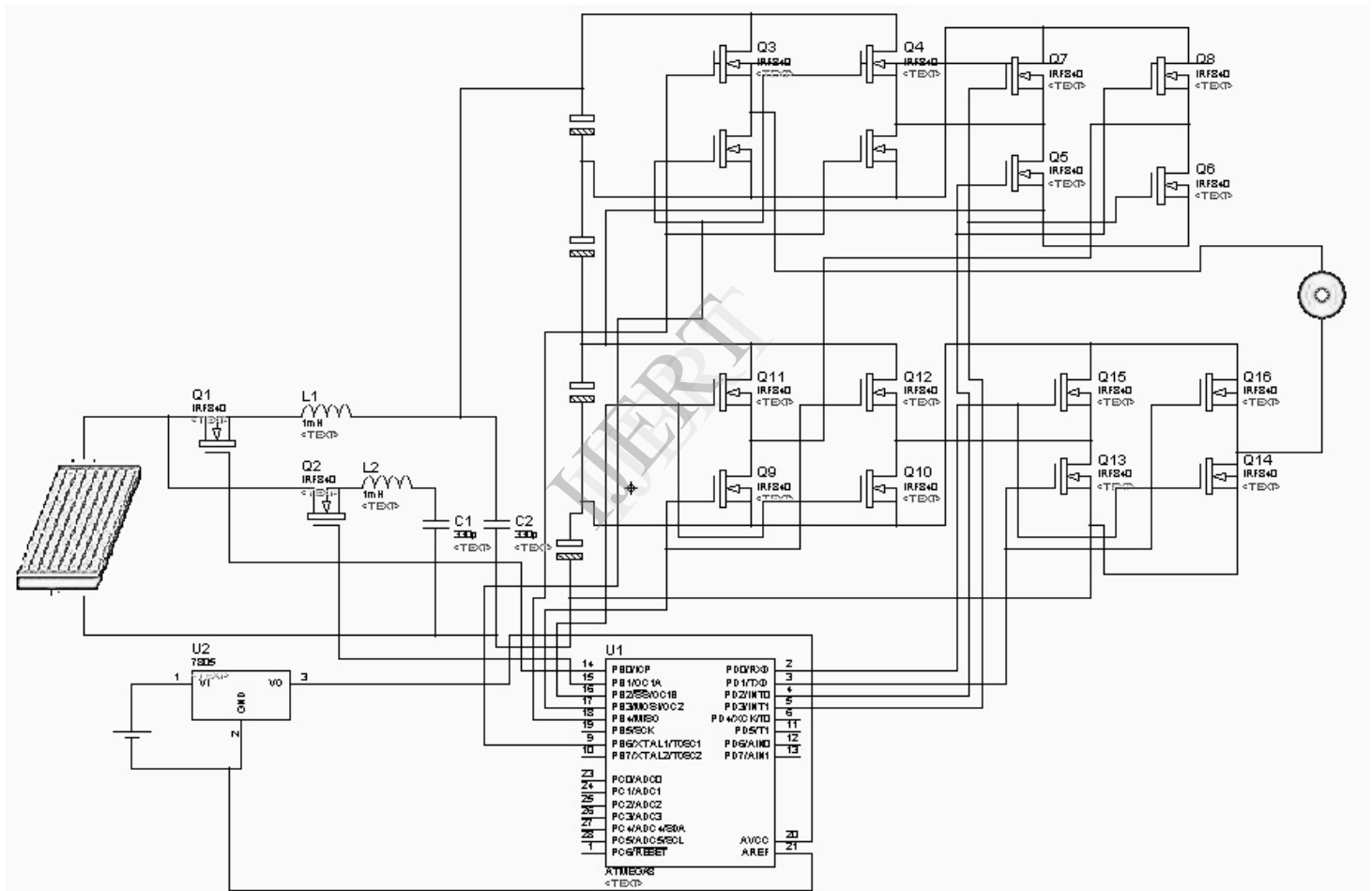
Fig 1 Circuit Diagram
