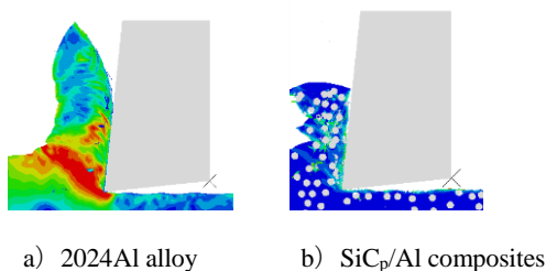
Fig.4 Simulation results of chip morphology
