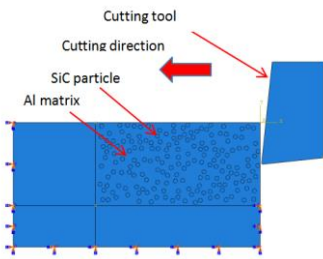
Figure 2 Boundary conditions and loading
