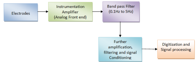
Figure 4 EOG Acquisition system for eye movement detection
