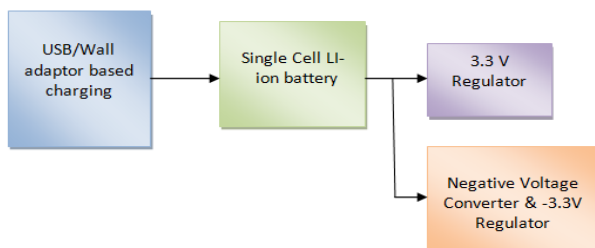
Figure 3 Power System for EOG based eye movement detection system
