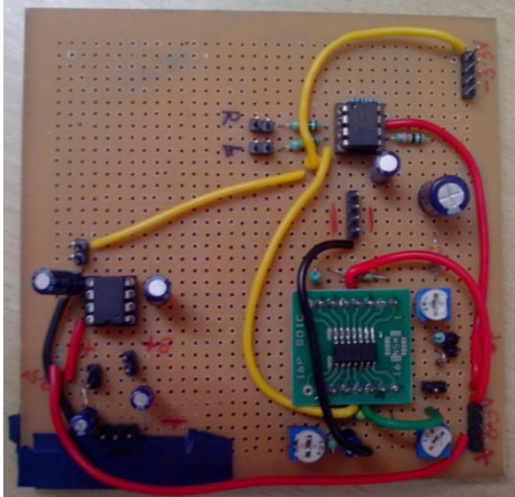
Figure 6 EOG analog circuitry
