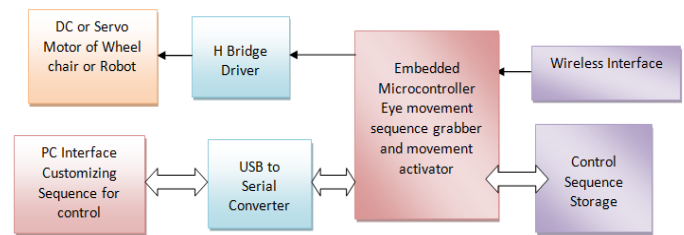
Figure 5 Eye movement Sequence identifier and motion control system
