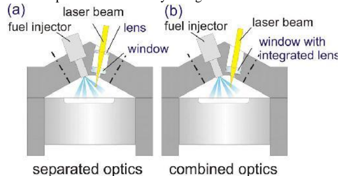
Fig. 2: Schematic cross section of the engine for laser ignition test runs. Two window/lens configurations were tested:
