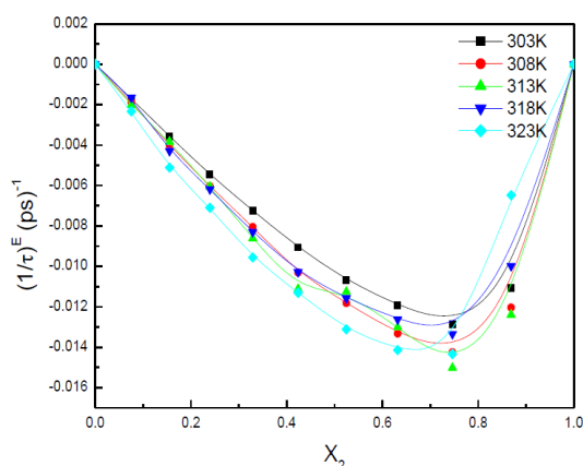
Fig.9. Plot of excessive relaxation time ((1/\tau)^E, \text{ps}^{-1}) with respective mole fraction of methyl benzoate in isobutanol ( X_2 ) at different temperatures.
