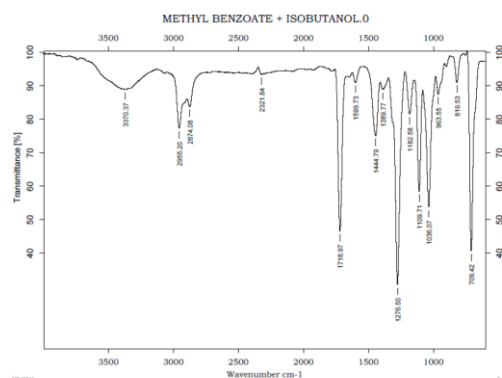
Fig.13. FT-IR sp-1ectra of the binary mixtures of Isobutanol and Methyl benzoate in the region of 450\text{--}4000\text{cm}^{-1}
