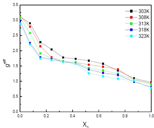
Fig.10. Plot of Kirkwood effective ( g^{\text{eff}} ) correlation factor with respective mole fraction of methyl benzoate in isobutanol ( X_2 ) at different temperatures
