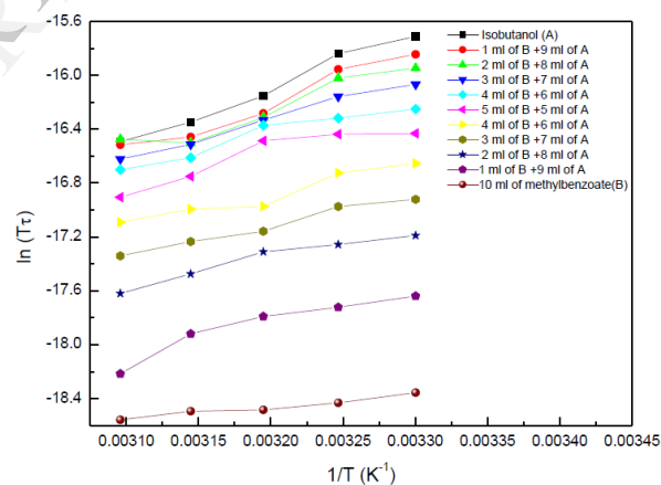
Fig.12. Plot of temperature dependence of \ln(T\tau) vs 1/T ( \text{K}^{-1} ) of different molar concentrations of methyl benzoate in isobutanol ( X_2 ) at different temperatures
