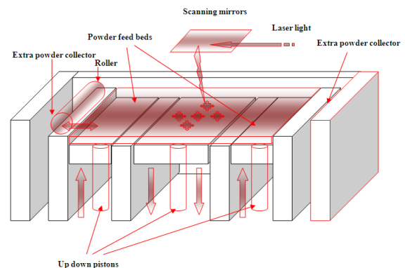
Figure: 1 Block diagram of Selective laser Sintering (SLS) process
