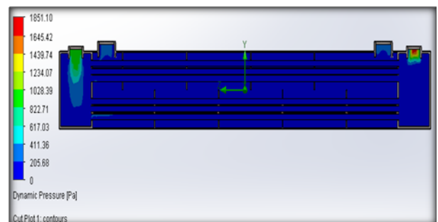
Fig. 4.2: Dynamic Pressure Plot of Smooth Tube HX
