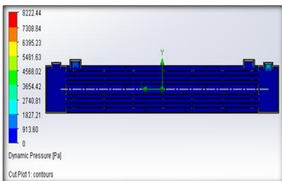
Fig. 4.6: Dynamic Pressure Plot of Corrugated Tube HX
