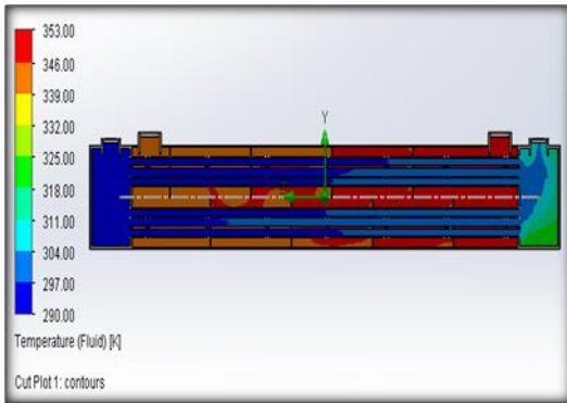
Fig. 4.3: Temperature Plot of Finned Tube HX
