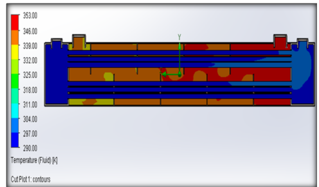
Fig.4.1: Temperature Plot of Smooth Tube HX
