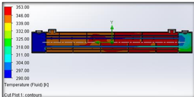
Fig. 4.5: Temperature Plot of Corrugated Tube HX
