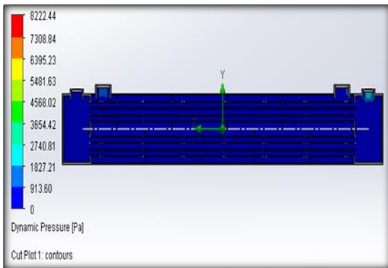
Fig. 4.4: Dynamic Pressure Plot of Finned Tube HX
