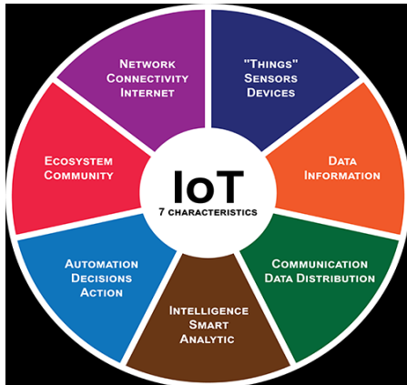
Fig. 3. IoT Characteristics
