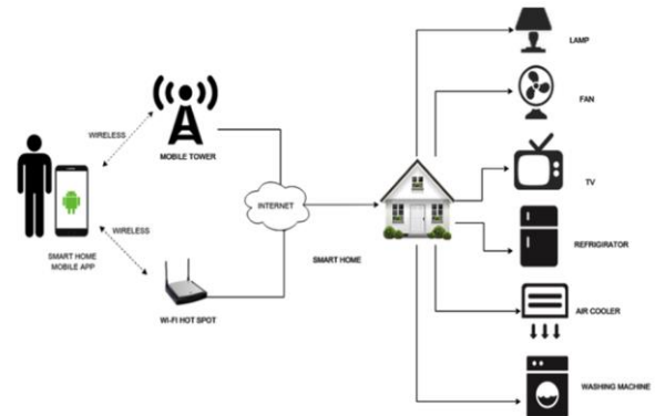
Fig. 7. Smart home
