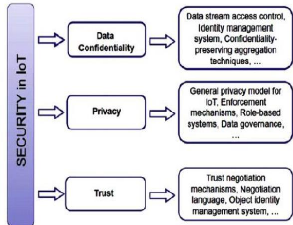
Fig. 10. IoT Security
