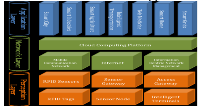
Fig. 4. IoT Architecture
