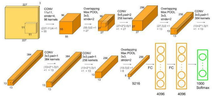
Figure 4: AlexNet Architecture
