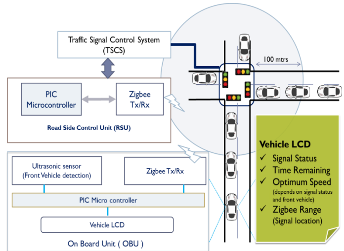
Fig. 2 Overview of predictive traffic light system
