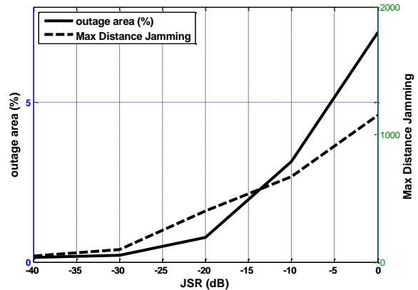
Fig. 4. The influence of the jammer's power on both the outage probability and the maximum coverage distance in a cluster that have one jammer when the jammer is fixed on the boarder of the cell.
