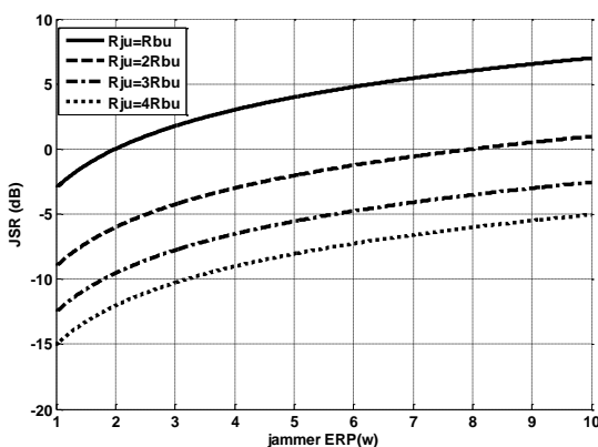
Fig. 3. The relation between the P_j(W) and JSR as (1).
