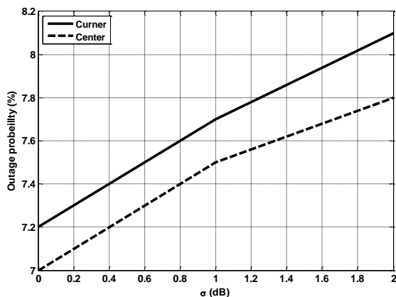
Fig.6effect of shadowing on the coverage area
