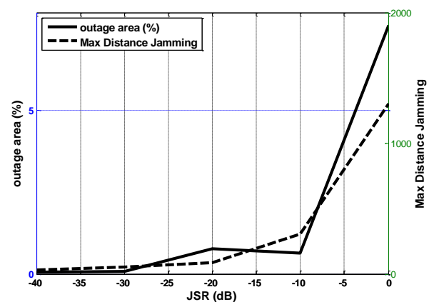
Fig. 5. The influence of the jammer's power on both the outage probability and the maximum coverage distance in a cluster that have one jammer when the jammer is close to the center of the cell.
