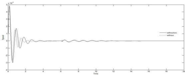
Fig 4 comparison of speed with and without SVC a) wm1-wm3 b) wm1-wm2
