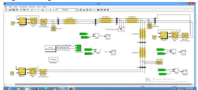
Fig2. Simulink model of 3 machine 9 bus system
