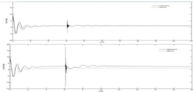
Fig 5 Comparison of load angle with and without SVC a) Delta 1 b) Delta 3
