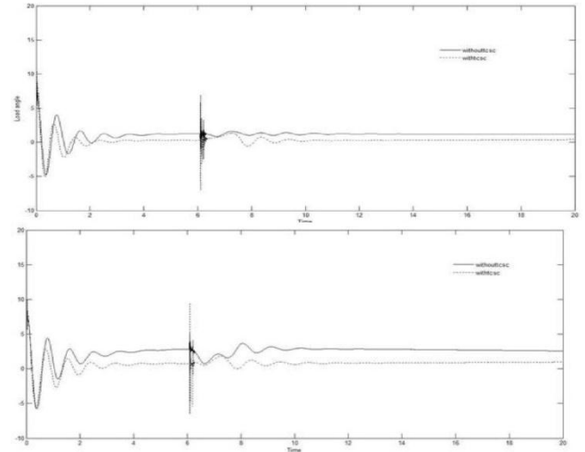
Fig 8 Comparison of Load angle with and without TCSC a) wm1-wm3 b) wm1-wm2
