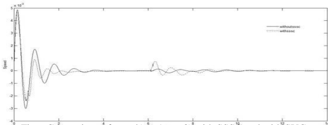
Fig 6 Comparison of speed(wm1-wm3) with SSSC and with SVC
