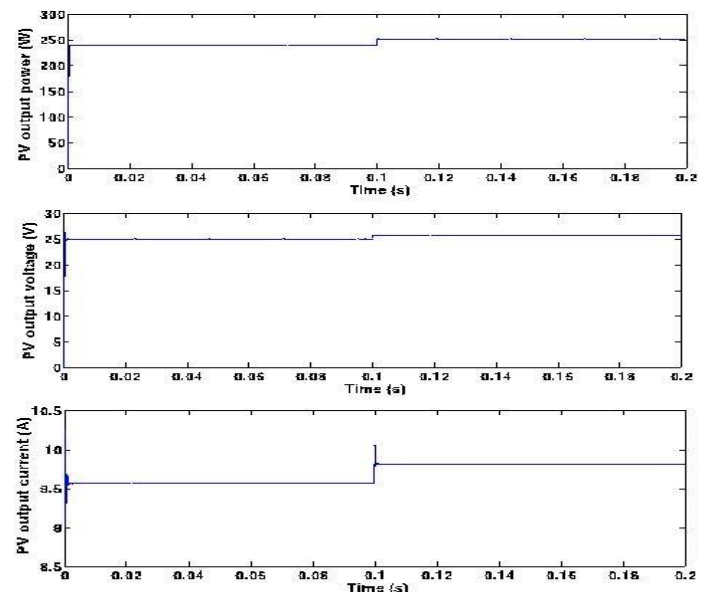
Fig.6. GWO-based MPPT.
