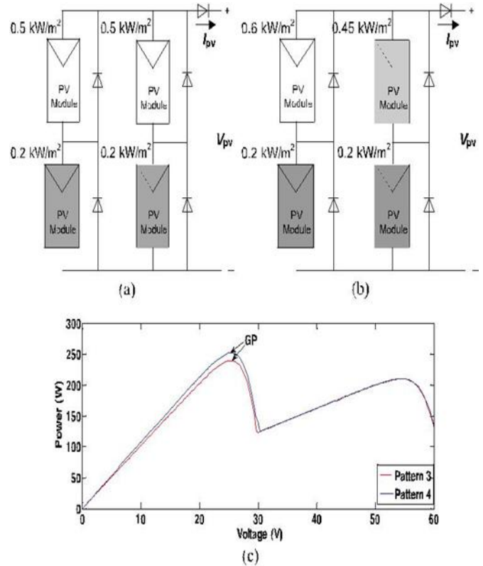
Fig.2. 2S2P configuration under different shading patterns. (a) Pattern 3.(b) Pattern 4. (c) P–V curves under PSCs.
