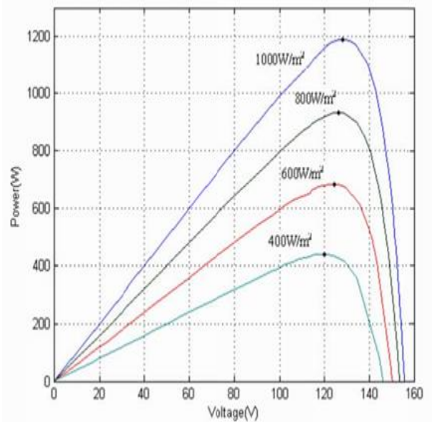
Fig.4.PVcurveofsolararrayfordifferentirradiationandconstante mperatureof25`C
