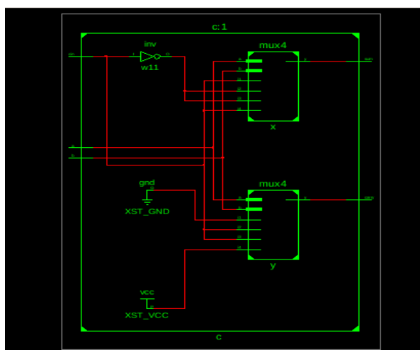
Figure 10. RTL Schematic of Full Adder using 4 by 1 MUX (FA2)
