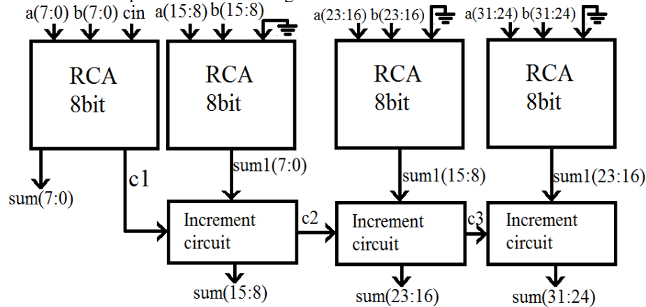
Figure 6. 32-Bit Carry Increment Adder (CIA)
