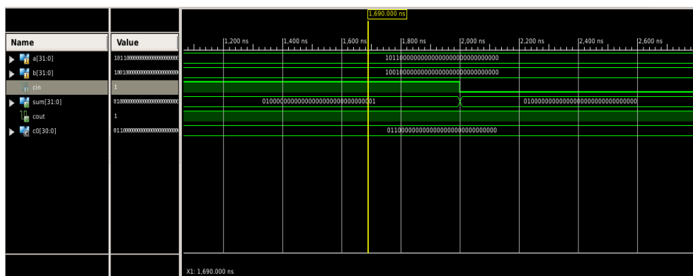
Figure 13. Simulation result of 32-bit Ripple Carry Adder (RCA)
