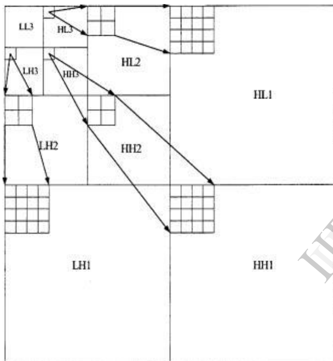
Figure 1 parent child relationship in SPIHT
