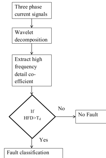
Figure.2. Block diagram of detection algorithm
