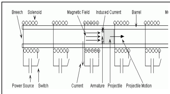
Fig. 4 Coil Gun Schematic
