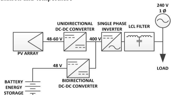
Fig 1 Circuit diagram for conventional method
