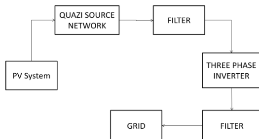
Fig 3 Block diagram of HPWM Three-Phase QZS Grid-Tie PV Power System
