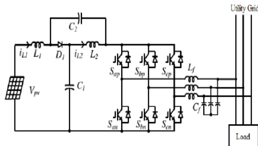
Fig. 2 Circuit diagram for proposed method
