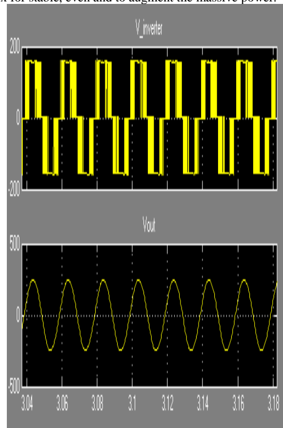
Fig 7 Inverter voltage & Output voltage
