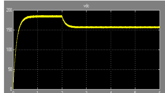
WAVEFORM FOR QZSI OUTPUT
