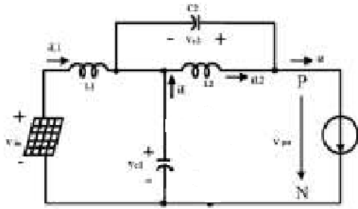
Fig 5 Mode of operation
