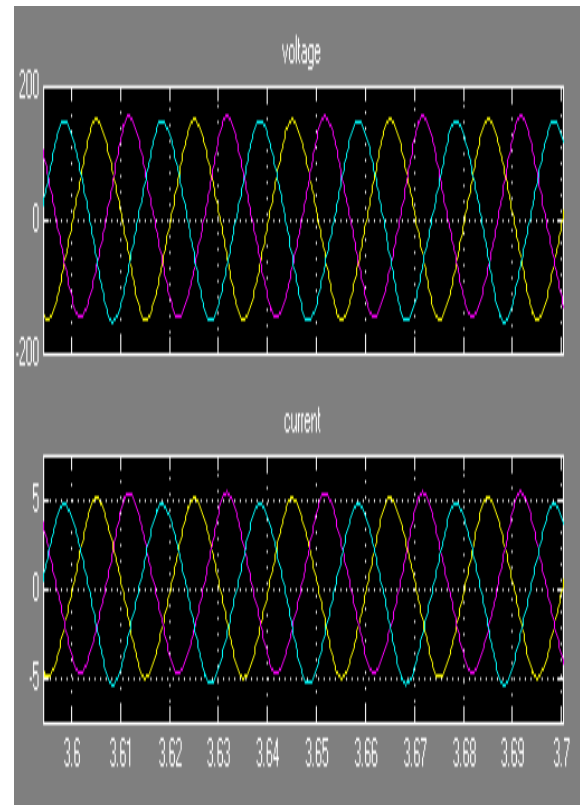
Fig 8 Grid voltage and current
