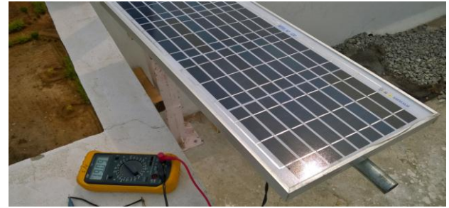
Fig 6.1.a: Solar panel output checking with multimeter
