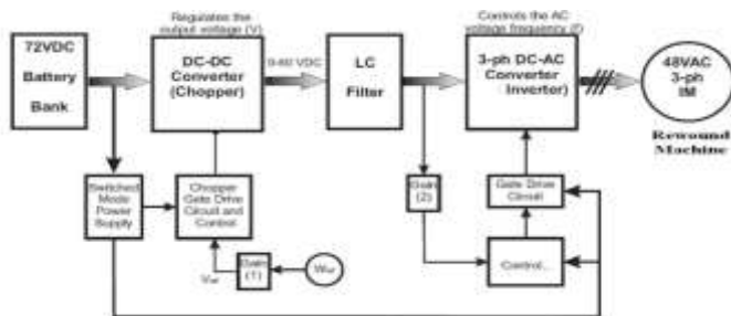
Fig.2. Block diagram of the entire proposed drive system
