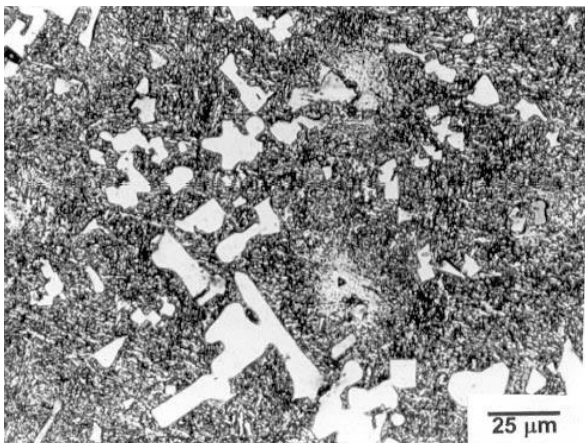
Fig. 1. Optical microstructure of the in-situ precipitated TiC in the matrix of Fe-Mn alloy for the sample A3.
