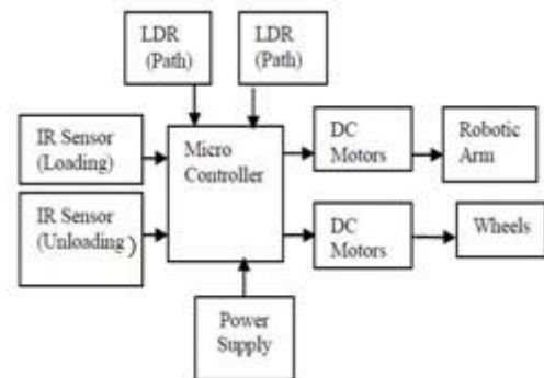
Fig.1 Block Diagram of the Guided Vehicle
