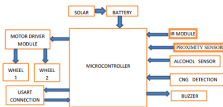
FIG 1. HARDWARE MODULE
