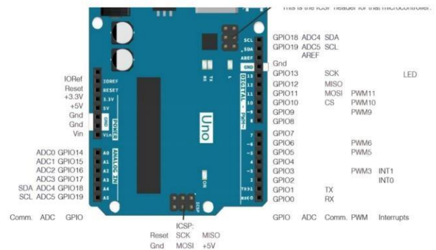
FIG 3. PIN DIAGRAM
