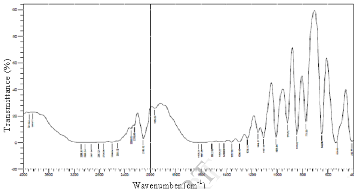
Figure 4. FTIR spectrum of LAMC
