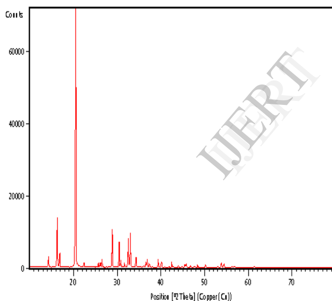
Figure 3. Powder X-ray diffraction pattern for LAMC.
