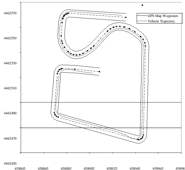
The X-axis of the graphic represents the East UTM Figure 3. Schematic representation of an automatic road tracking based on fuzzy logic and GPS.
