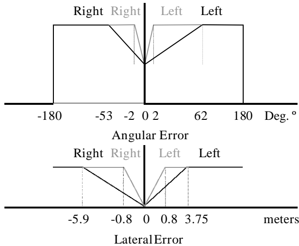
Figure 2. Angular and Lateral error membership functions
