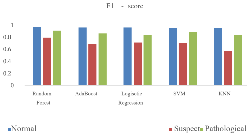
Figure 4: F1-score of models in proposed solution
