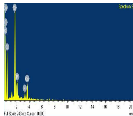
Figure 3: Edx Spectrum For RHA
