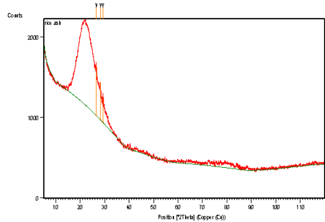
Figure 7 XRD Plot for RHA
