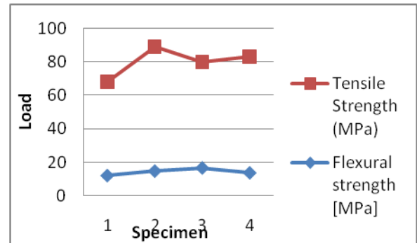
Graph 5.7 Comparison of Flexural and Tensile strength for different specimens
