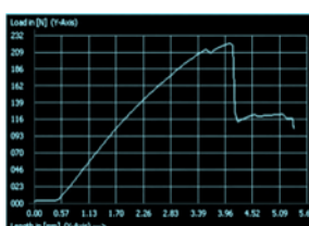
Graph 5.3 Flexural test on sample 4 Specimen
