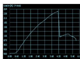
Graph 5.2 Flexural test on sample 2 Specimen
