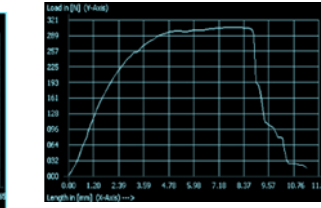
Graph 5.4 Flexural test on sample 3 Specimen
