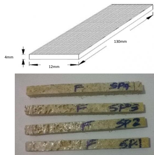
Fig 4.2 Flexural test specimens
