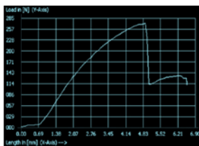
Graph 5.1 flexural test on sample 1 specimen
