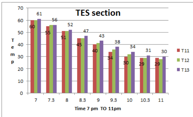
Fig 15: Outlet air temperatures vs. time
