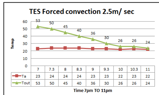
Fig 13: Outlet air temperatures vs. night time
