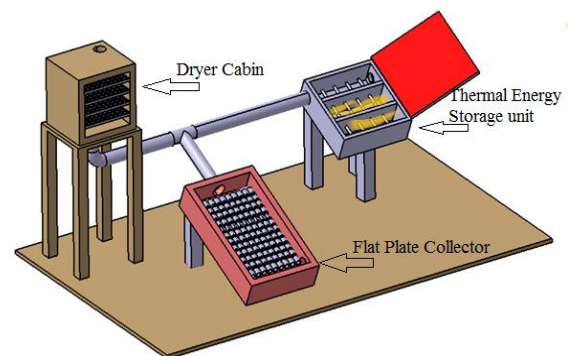
Fig 2: Experimental setup.
