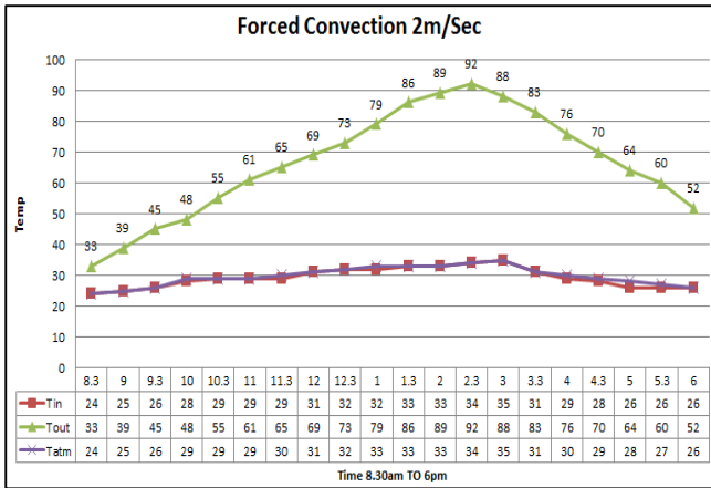
Fig 8: Outlet air temperatures vs. time (2 m/ sec)
