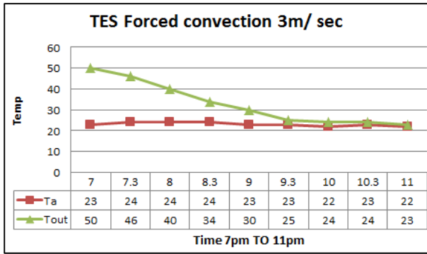
Fig 14: Outlet air temperatures vs. night time
