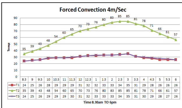
Fig 10: Outlet air temperatures vs. time (4 m/ sec)
