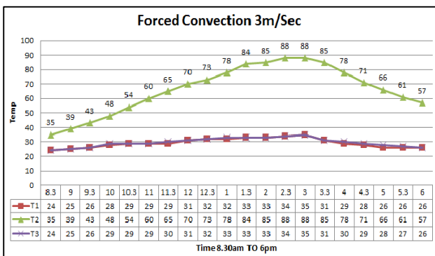
Fig 9: Outlet air temperatures vs. time (3 m/ sec)
