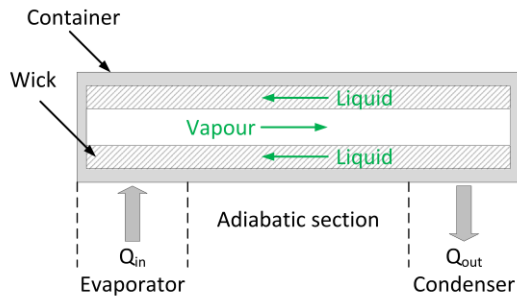
Fig.5. Working Principle of Heat Pipe.
