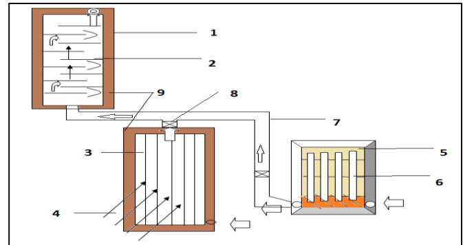
Fig 1: Solar air dryer: (1) Storage, (2) trays, (3) FPC, (4) Solar rays, (5) PCM, (6) Heat pipe, (7) Piping, (8) Control valves, (9) Insulation
