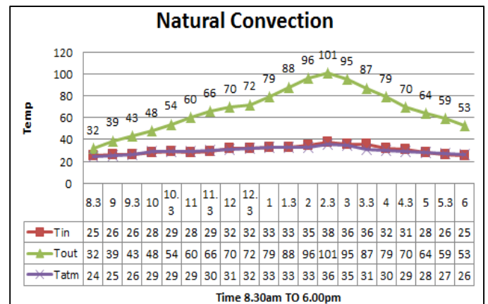
Fig 7: Outlet air temperatures vs. time
