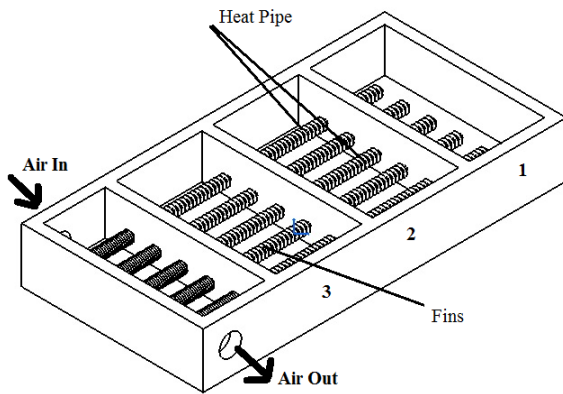
Fig 6: Schematics of LHTES unit; Five Heat pipe and Fin
