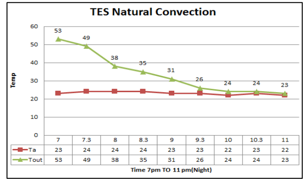
Fig 11: Outlet air temperatures vs. night time
