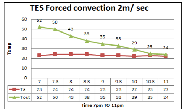
Fig 12: Outlet air temperatures vs. night time
