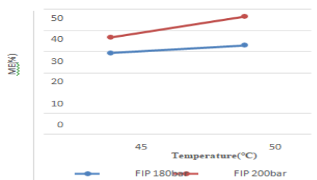
Fig. 5. Mechanical efficiency (%) vs Temperature(°C)
