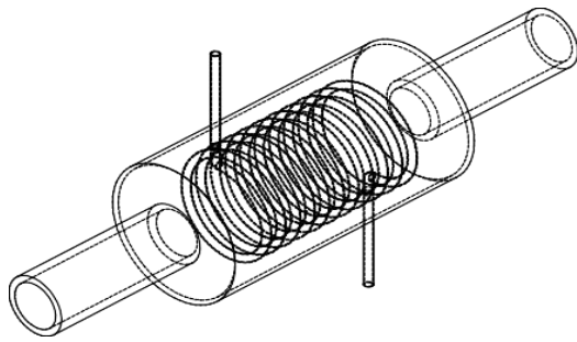
Fig. 1. 2D view of a pre-heating chamber
