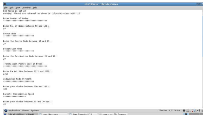
Fig. 4. Input of simulation
