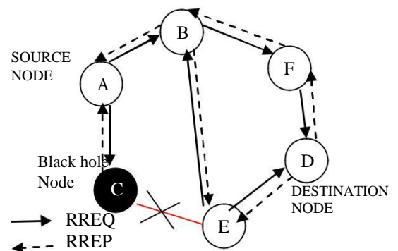
Figure.2. Black hole node in AODV
