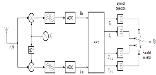
2 (b): Block diagram of OFDM-MIMO (STC) Receiver System.
