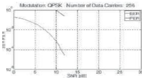
Fig.8: Performance of a QPSK modulation for without padding Parameters: No. of FFT points =256; Modulation = QPSK; Channel = AWGN, Tx elements=2 and Rx element =2.
