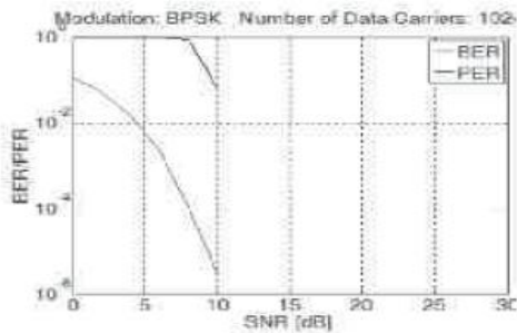
Fig.7: Performance of a BPSK modulation for without padding Parameters: No. of FFT points = 1024; Modulation = BPSK; Channel = AWGN, Tx elements=2 and Rx element =2.
