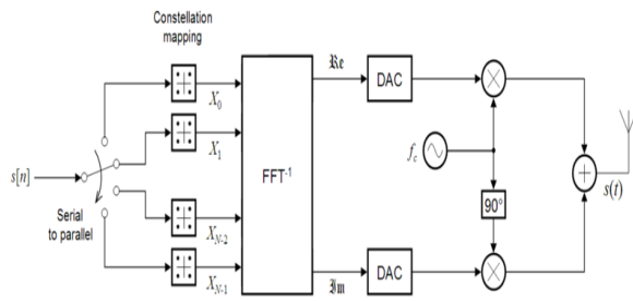
2 (a): Block diagram of OFDM-MIMO (STC) Transmitter System.
