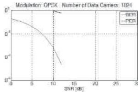
Fig.9: Performance of a QPSK modulation for without padding Parameters: No. of FFT points = 1024; Modulation = QPSK; Channel = AWGN, Tx elements=2 and Rx element =2.
