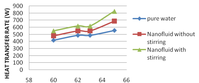
INLET TEMPERATURE Vs HEAT TRANSFER RATE
