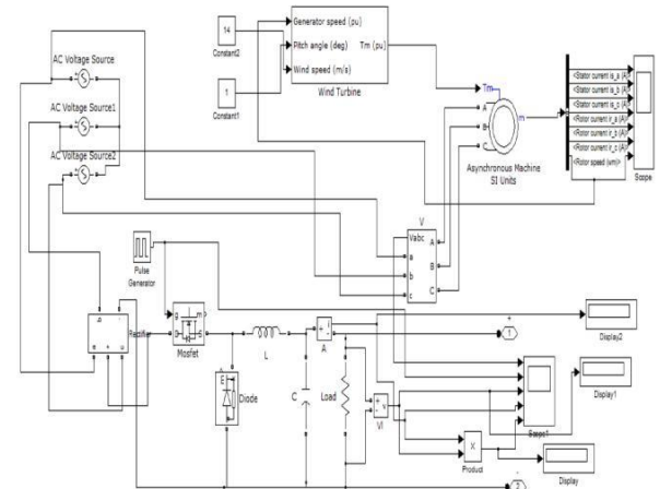
Fig. 8 Simulation diagram of wind energy Conversion system
