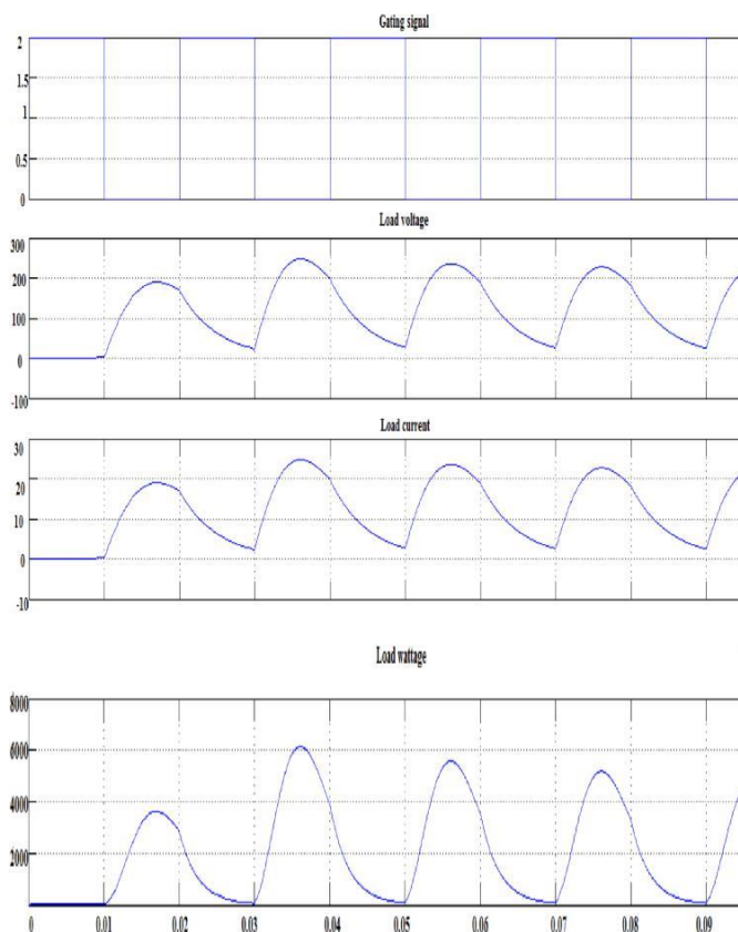
Fig. 11 Output waveform of Diesel power generation system.
