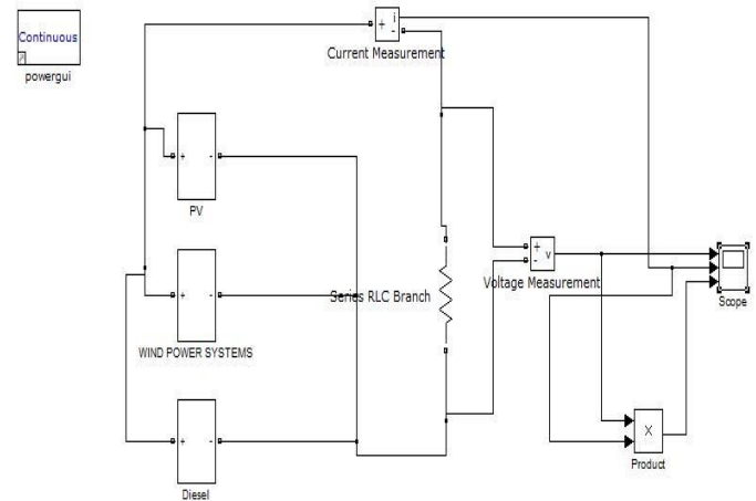
Fig. 12 Simulation diagram of integrated system
