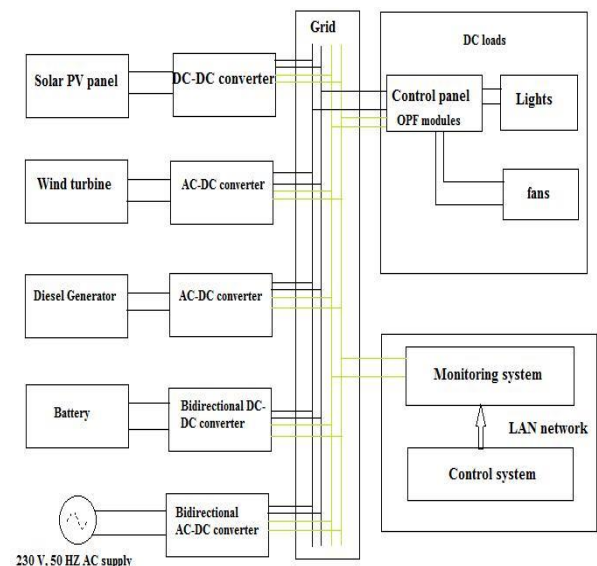
Fig. 1 Block diagram of the smart micro grid systems
