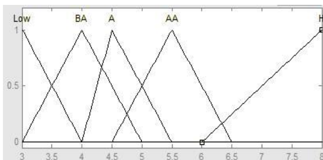
Fig. 4(a) Input membership function P_e
