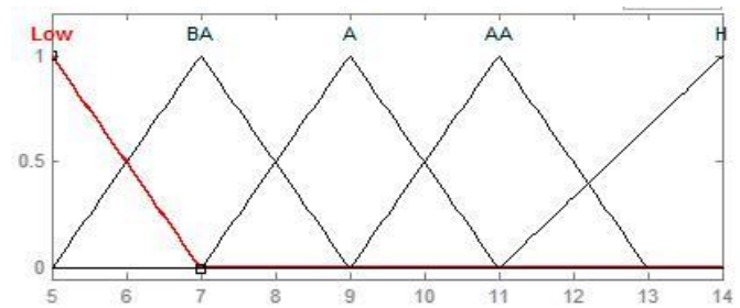
Fig. 4(c) Output membership function I_c .
