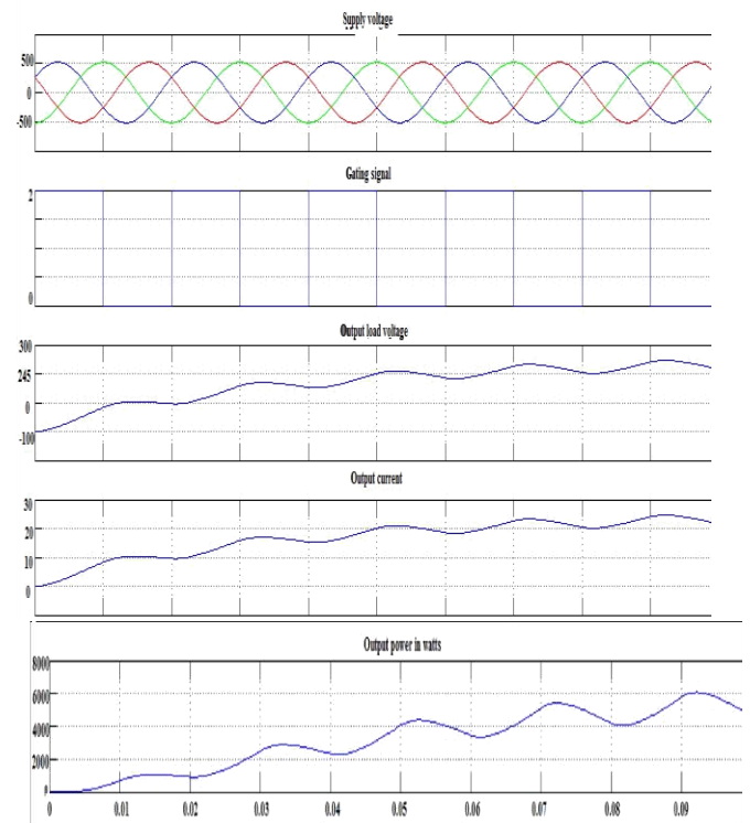
Fig. 9 Output waveform of Wind energy Conversion system.
