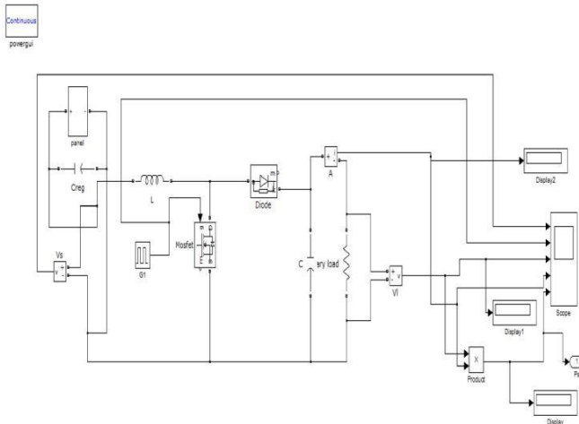
Fig. 6 Simulation Circuit diagram of PV system.
