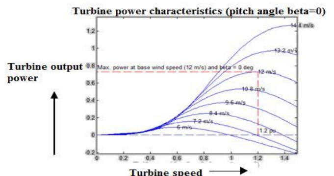
Fig. 3 Characteristics of Wind turbine
