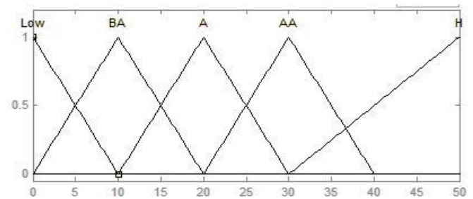
Fig. 4(b) Input membership function \text{SOC}_e .
