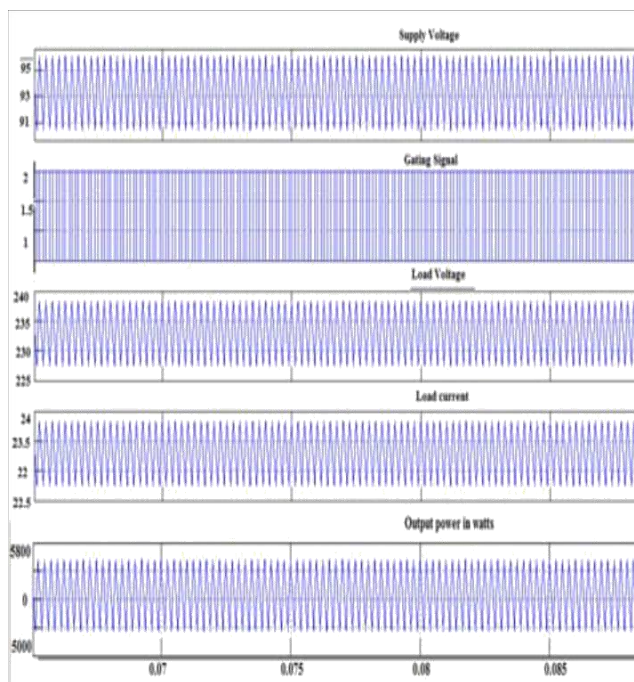
Fig. 7 Output waveform of PV system.
