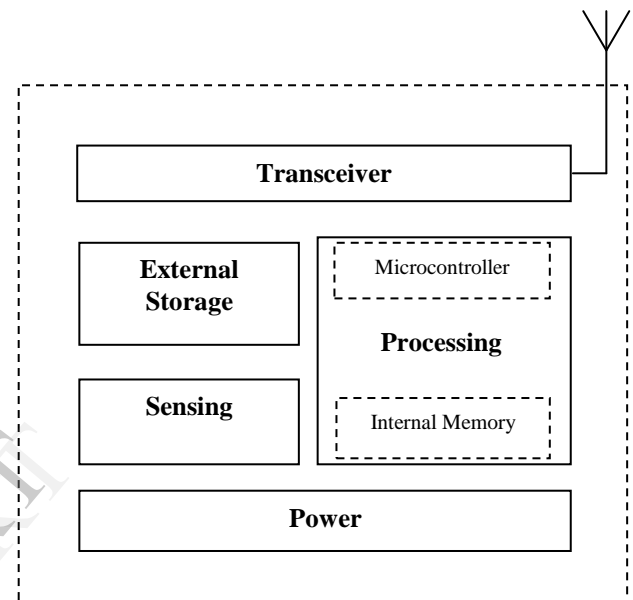
Fig.2. 1 Main Components of a Sensor Node
