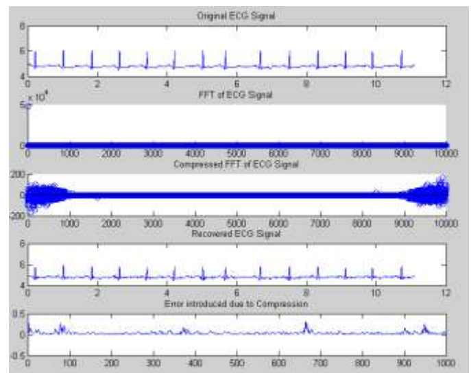
Fig 4: Actual ECG signal compressed using FFT algorithm
