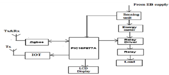
Fig.- 4.Receiver1Block Diagram
