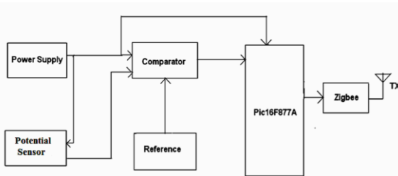
Fig.- 3.Transmitter Block Diagram
