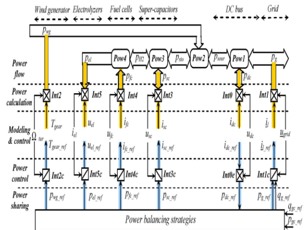
Fig. 4. Multilevel representation of the power modeling and control of the HPS.
