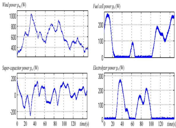
Fig. 10. Power profiles of the different sources.
