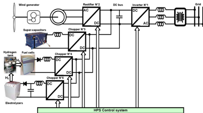
Fig. 1. Structure of the studied wind/hydrogen/SC HPS.
