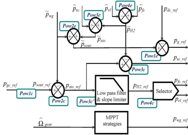
Fig. 6. Block diagram of the grid-following strategy.
