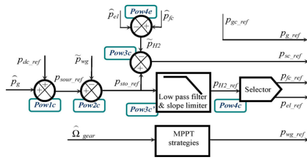
Fig. 8. Block diagram of the source-following strategy.
