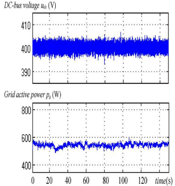
Fig. 11. Grid-following strategy test results.
