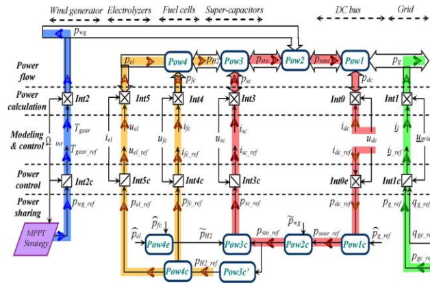
Fig. 7. Multilevel representation of the source-following strategy
