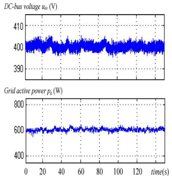
Fig. 12. Source-following strategy test results.
