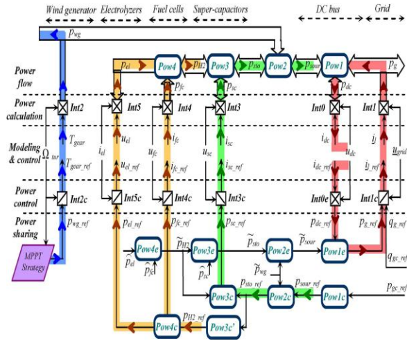
Fig. 5. Multilevel representation of the grid-following strategy.
