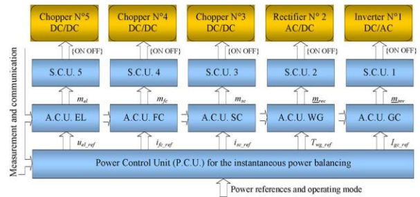
Fig. 2. Hierarchical control structure of the HPS.
