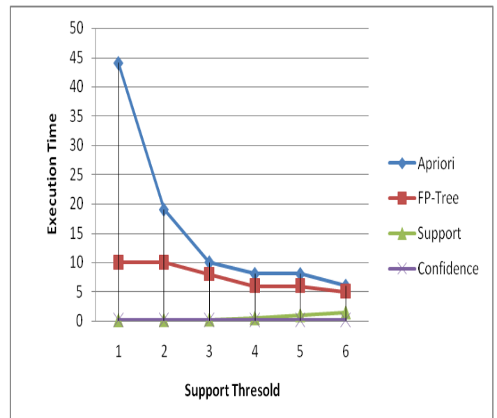
Figure 6. Comparison chart performance of Apriori and Fp-Tree based on support and confidence
