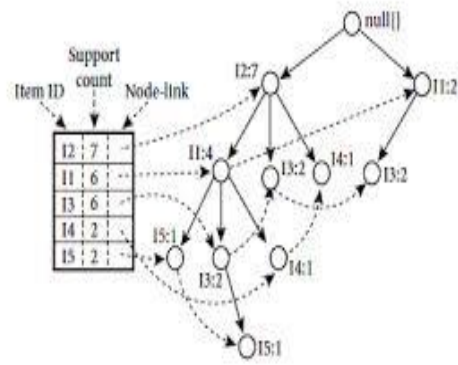
Figure 5. FP-Tree
